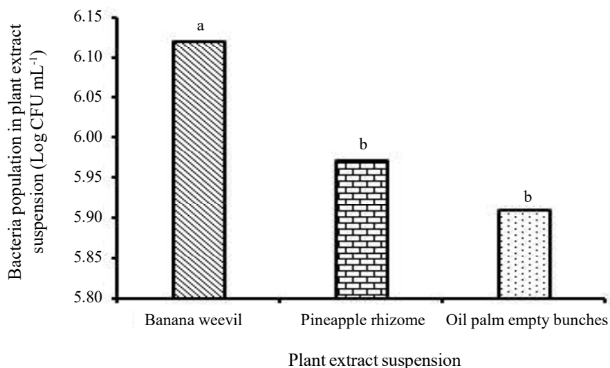
Figure 1. Total of bacteria population in plant extract suspension. The same letter on the bar shows no significant difference based on the DMRT test at the 5% level.
