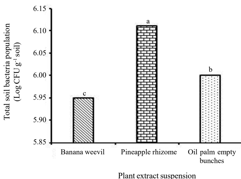
Figure 3. Bacteria population in the soil-applied with plant extract suspension. The same letter on the bar shows no significant difference based on the DMRT test at the 5% level.
