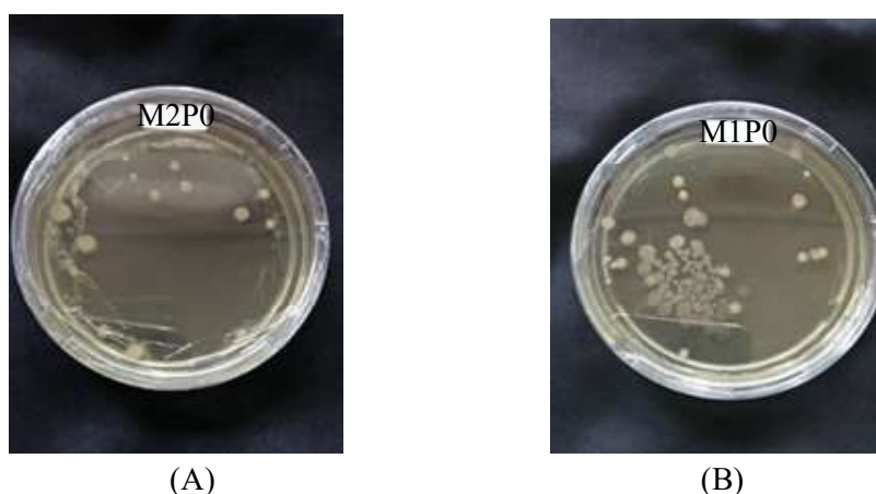
Figure 4. Soil bacterial population isolated from soil that has been applied by plant extract suspension; suspension extracts from pineapple rhizome (A); suspension extract from banana weevil (B).
