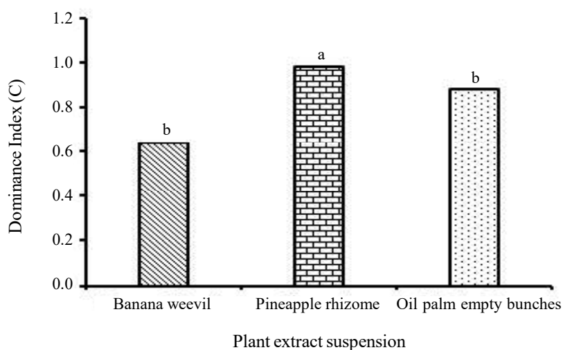
Figure 6. Mesofauna dominance index in soil with plant extract suspension. The same letter on the bar shows no significant difference based on the DMRT test at the 5% level.
