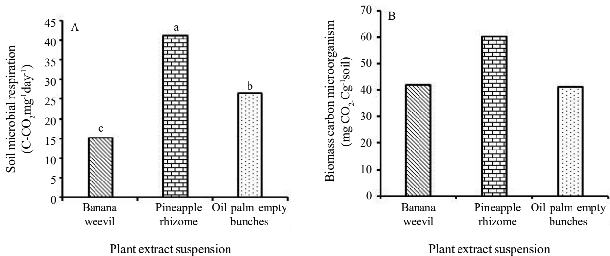
Figure 8. Improvement of soil microbial respiration (A); soil microbial carbon biomass (B) application of plant extract suspension. The same letter on the bar shows no significant difference based on the DMRT test at the 5% level.
