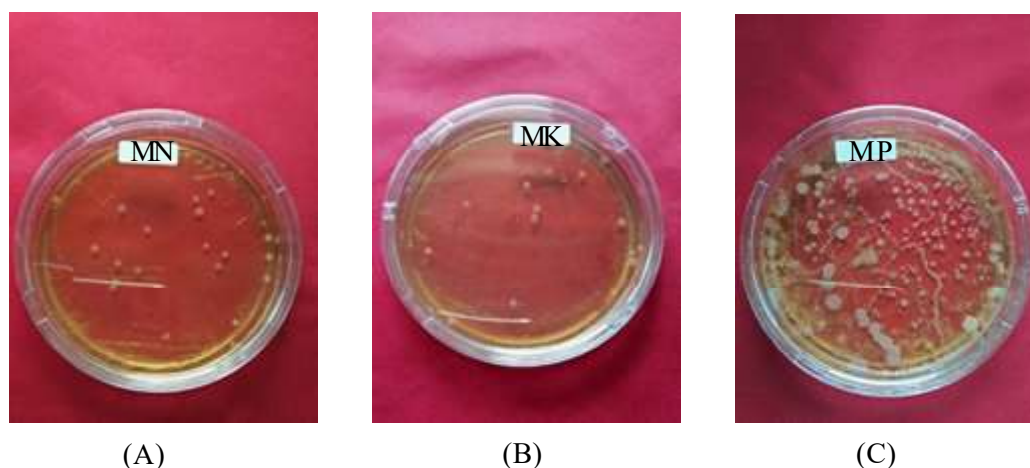
Figure 2. Bacterial colonies in the suspension of plant extract from pineapple rhizome (A), oil palm empty bunches (B), and banana weevil (C).
