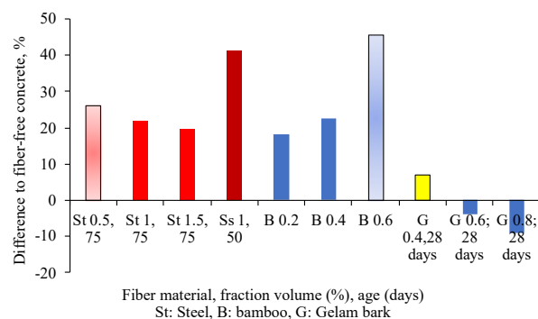
Figure 3. Splitting test
