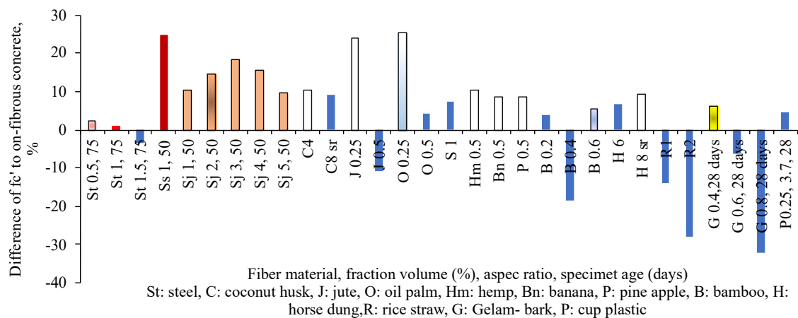
Figure 2. Compressive strength
