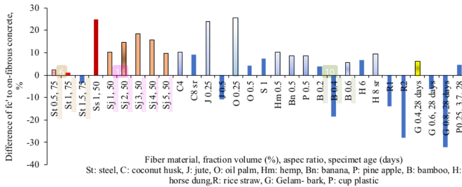
31 Figure 2. Compressive strength
