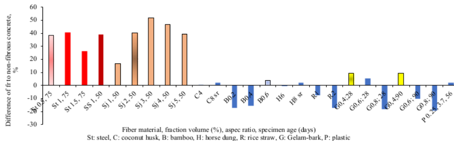
Figure 1. Modulus of rupture
