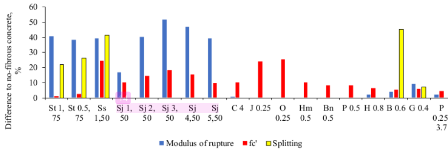
Figure 4. Improved mechanical properties of fibrous concrete
