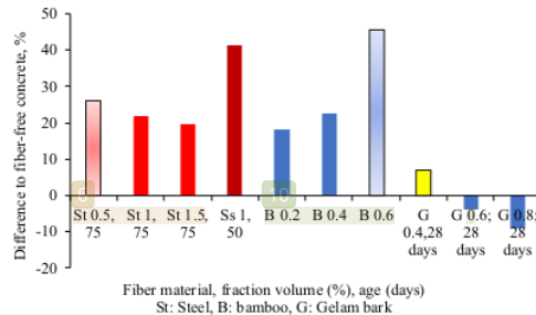
Figure 3. Splitting test
