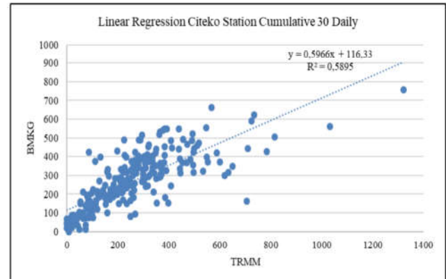
Figure 18. Linear Regression Graph Citeko Station Cumulative 30 Daily.
