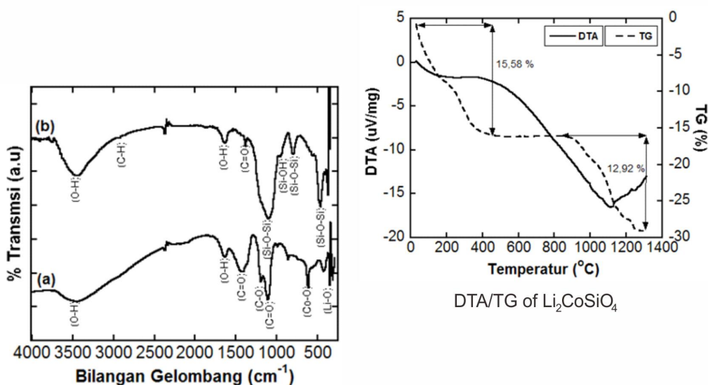
FTIR spectra of \text{Li}_2\text{CoSiO}_4 prepared from (a) battery cathode waste (b) rice husk ash silica
