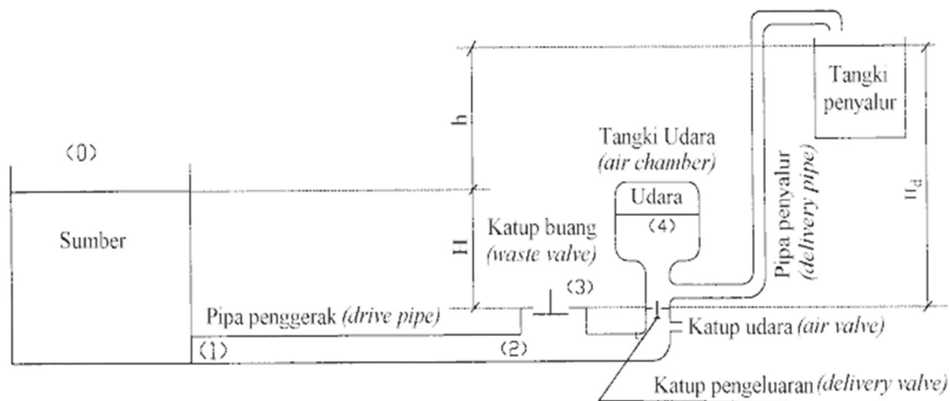
Gambar 1. Instalasi pompa hydraulic ram pump
