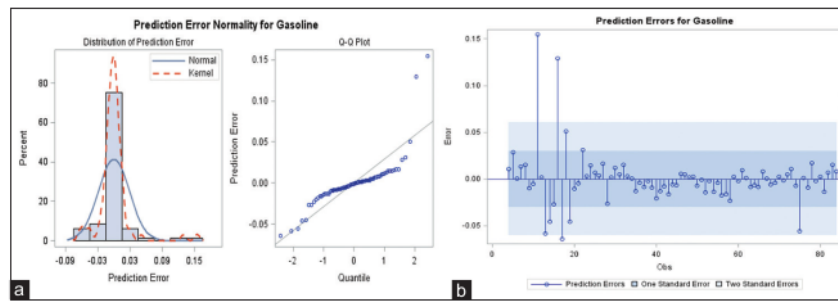
Figure 2: (a and b) Prediction error normality for data gasoline price
