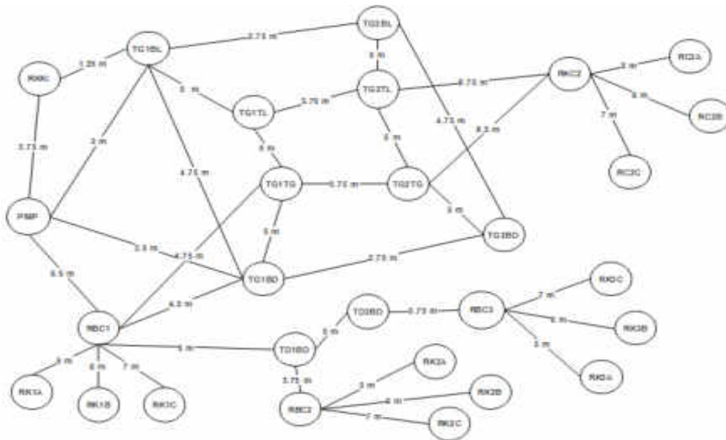
Gambar 6. Graph Diagram
