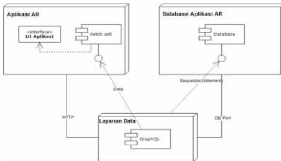
Gambar 14. Deployment Diagram
