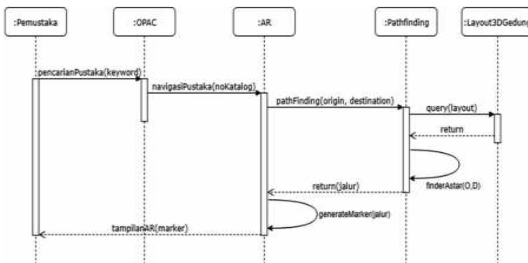
Gambar 4. Sequence Diagram
