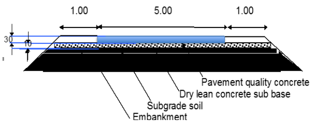
Fig.1. Cross section of the rigid pavement
