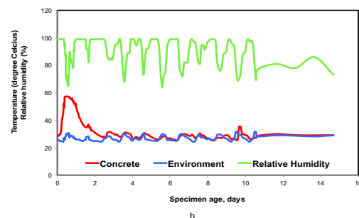
Fig. 8. Deformation of HPC rigid pavement, concrete and environmental temperature and relative humidity
