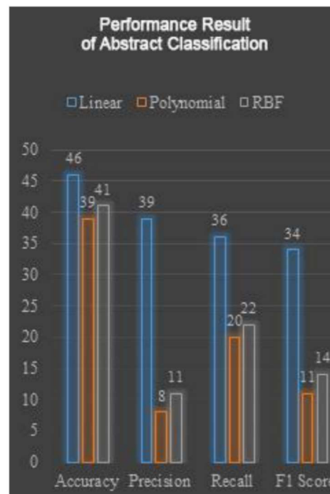
Figure 3. Comparison of classification performance using each kernels.
