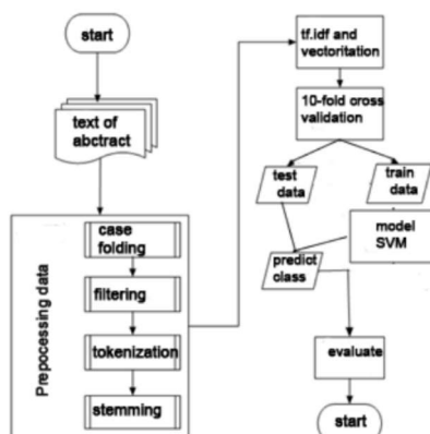
Figure 1. Flow chart of text classification in this research.
