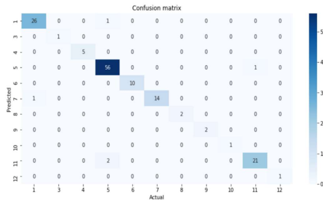
Figure 5. Confusion matrix of 205 important features.
