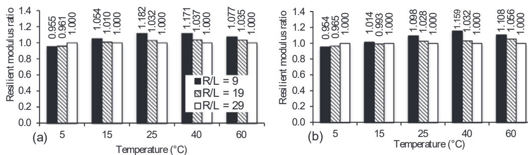
Fig. 5. Effect of rest period ratio on resilient modulus of (a) unmodified asphalt mixtures, (b) BRA modified asphalt mixtures.
