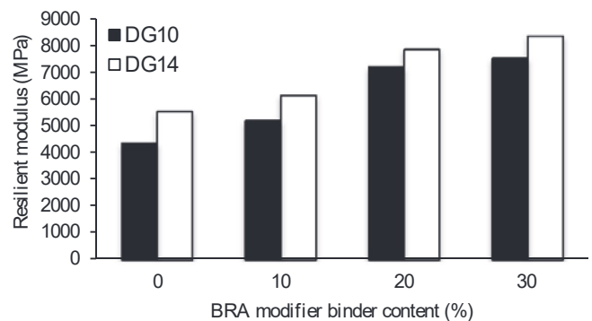
Fig. 3. Resilient modulus of unmodified and BRA modified asphalt mixtures.
