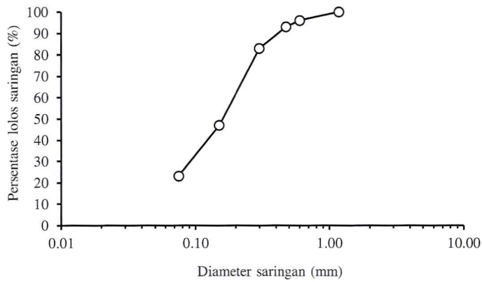
Gambar 2. Gradasi mineral Aspal Buton
