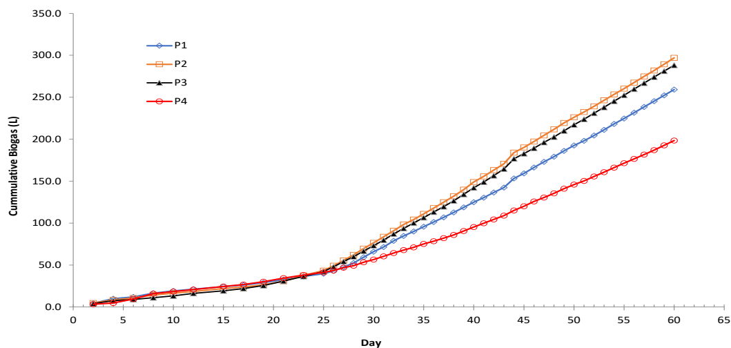
Figure 6. Cumulative biogas production from different treatment.
