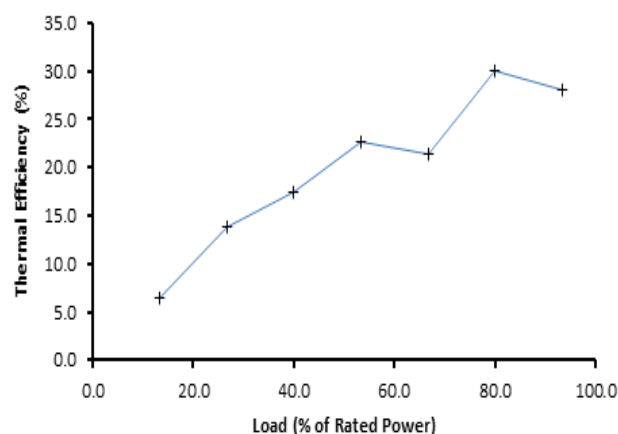
Figure 5. Effect of load on the thermal efficiency.
