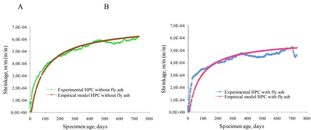
Figure 5. Experimental and empirical model of HPC 5A. Without fly ash (DB); 5B. With fly ash (TB).
