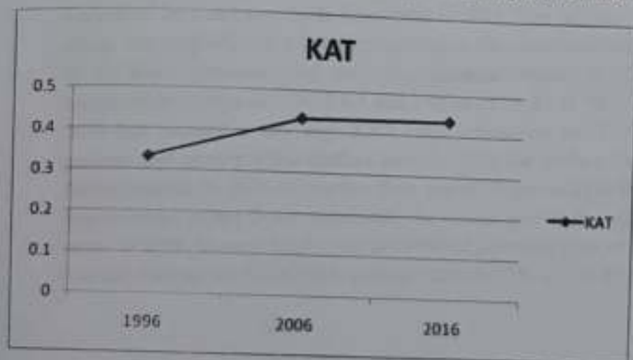
Figure 5. Graph of surface flow in the Bulok Sub-watershed
