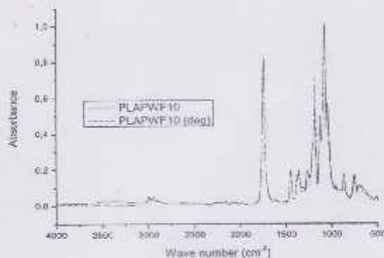
Figure 7. FTIR spectra of hydrolysis degradation of polylactide and polylactide with 10% MEP from wood flour before and after degradation 28 days, 370^{\circ}\text{C}
