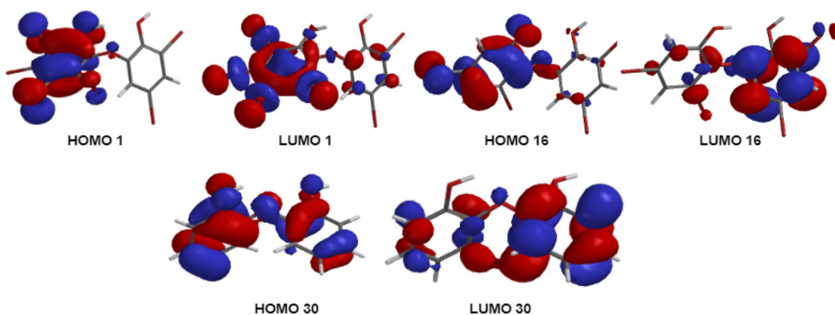
Figure 9. FMOs (HOMO and LUMO) for 1, 16, and 30.
