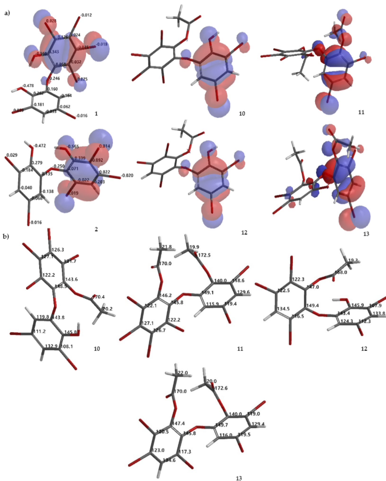
Figure 6. Molecular orbital analysis (HOMO) of 1, 2, 10–13 calculated using DFT \omega B97X-D/6–311 + G(2d,p) along with analysis of electrostatic charges of 1 and 2 (a). Proposed calculated ^{13}\text{C} NMR chemical shifts of 10–13 using the NMR chemical shift calculation protocol (b).
