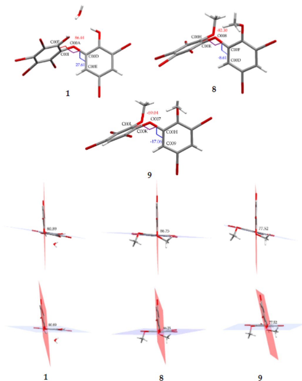
Figure 4. Torsion and dihedral angles of 1, 8, and 9.
