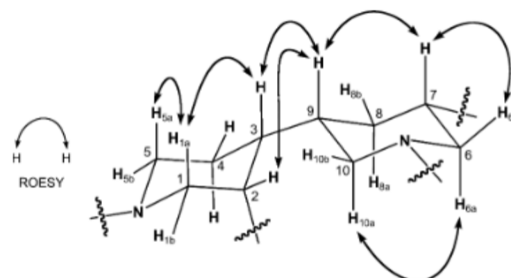
Fig. 3. ROESY Correlations for 1
