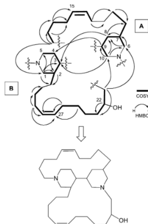
Fig. 2. COSY and HMBC Correlations for 1
