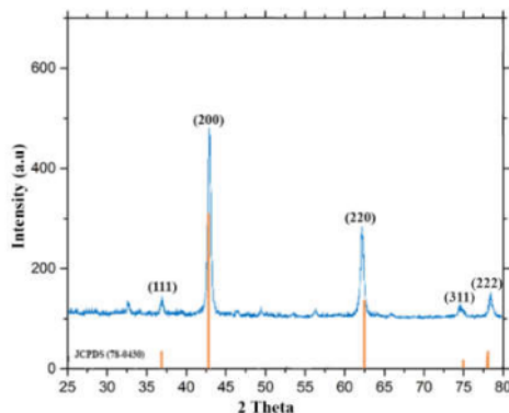
Figure 2. XRD pattern of MgO nanoparticles.
