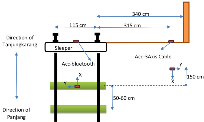
Figure 4. Sensors application on sleeper and ground
