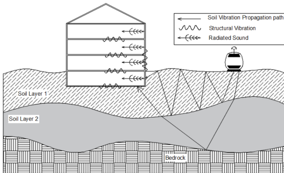
Figure 1. Vibration from train transferred to buildings [8]
