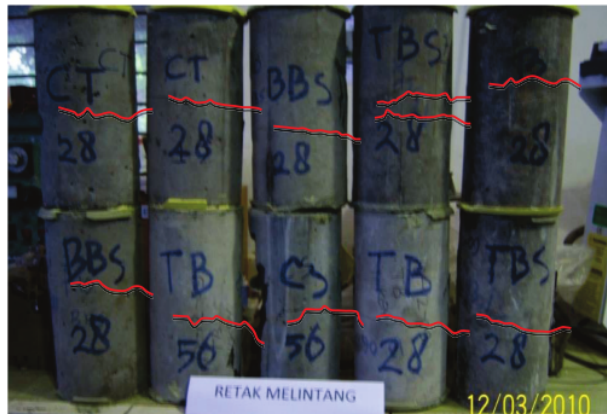
Fig. 5. Compression failure type of specimens with superplasticizer H
