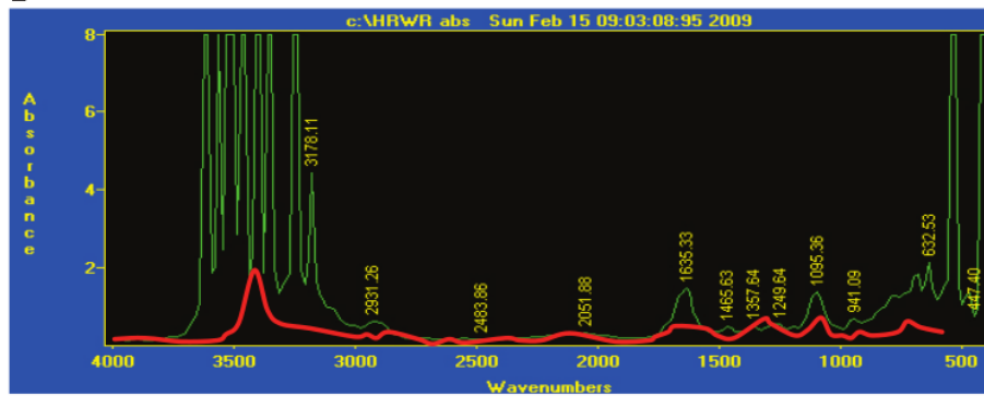
Figure 6. FT-IR graph or fingerprint of superplasticizer V and H
