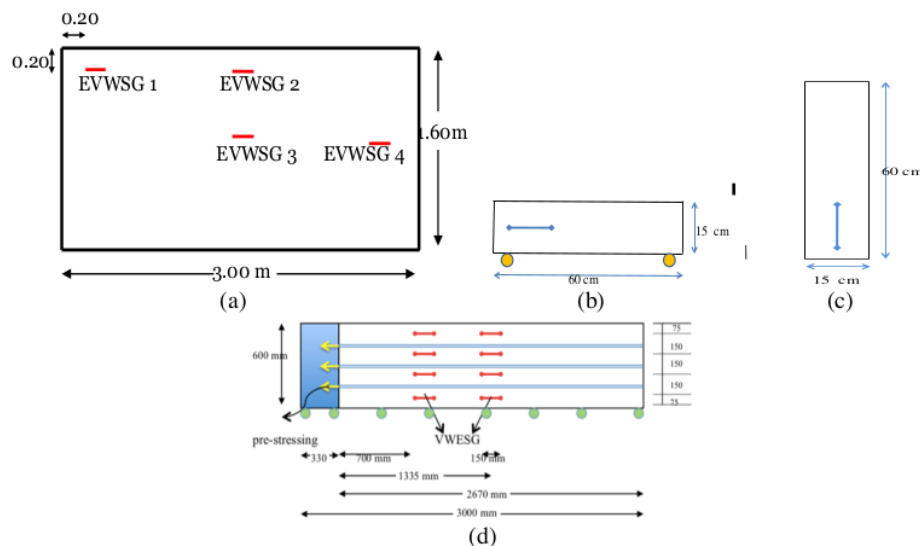
Figure 1. Specimens and placement of EVWSG: (a) Plate, (b) Laboratory-scale beam specimen, (c) Laboratory-scale column specimen, (d) Full-scale beam specimen
