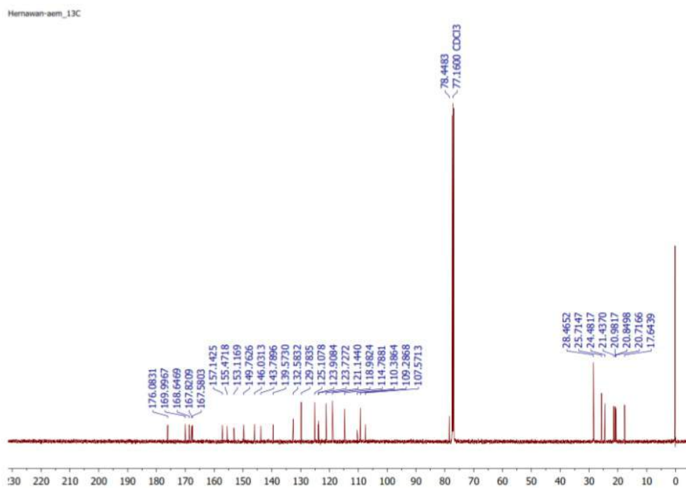
Fig. 4. ^{13}\text{C} NMR spectrum of compound I
