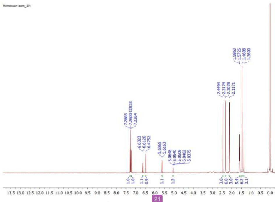
Fig. 3. ^1\text{H} NMR spectrum of compound I
