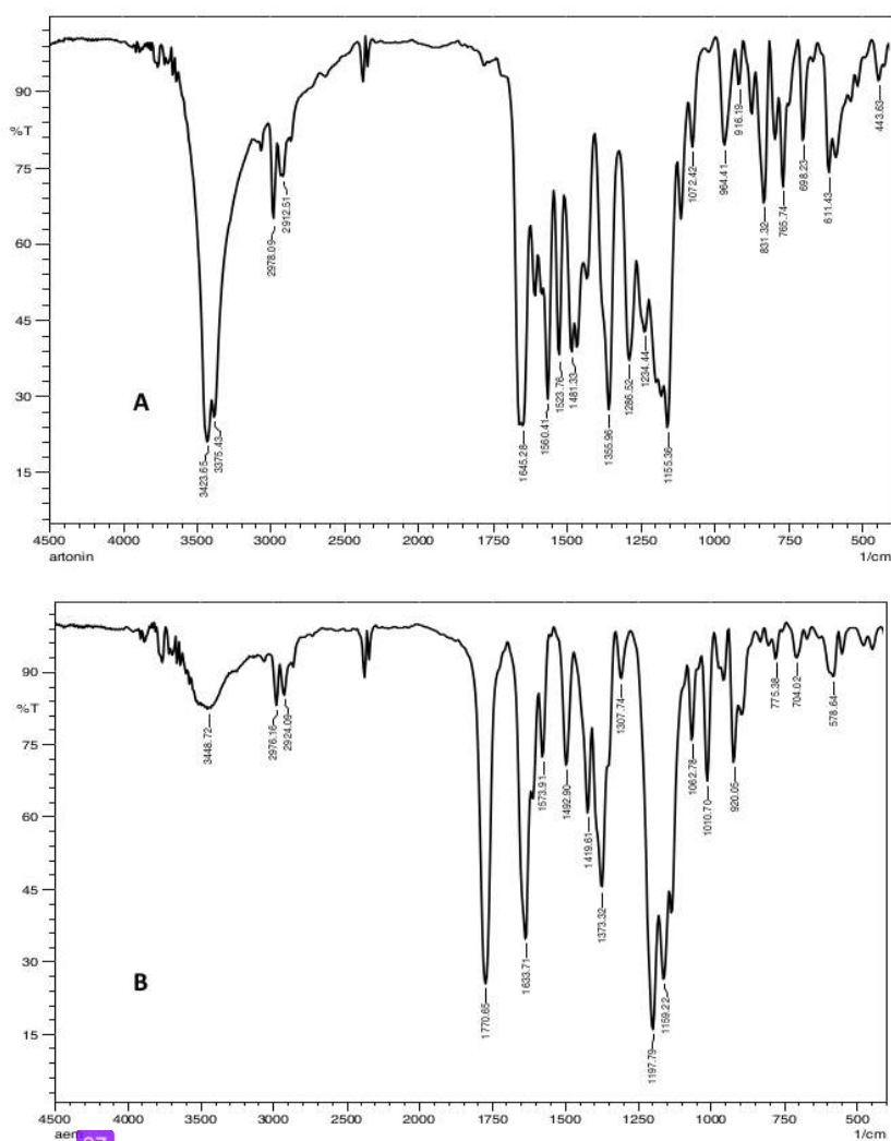
Fig. 2. The comparison of IR spectra of (A) isolated artonin E [1]; (B) compound 1
