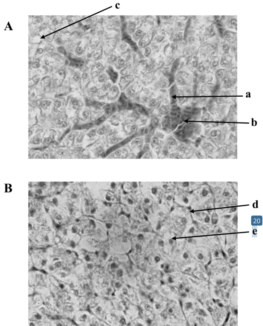
Figure 2. (A) Histological preparation of liver cells in Nile tilapia collected from WWTPs PT. Gunung Madu Plantation, Lampung, Indonesia (a) hyperemia (congestion) in the sinusoid or blood vessel cells in the small vena. (b) infiltration (cellular inflammation) near the vena centralist. and (c) fatty change in liver from fish in the first and second aeration WWTP. (B) Hepatocyte cell from fish in the control pond: (d) nuclei (e) membrane cell. HE X 400
