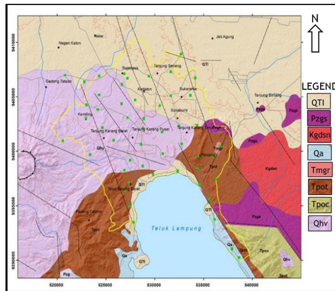
FIGURE 1. Geological Map of Bandar Lampung [10] modified from [9].
