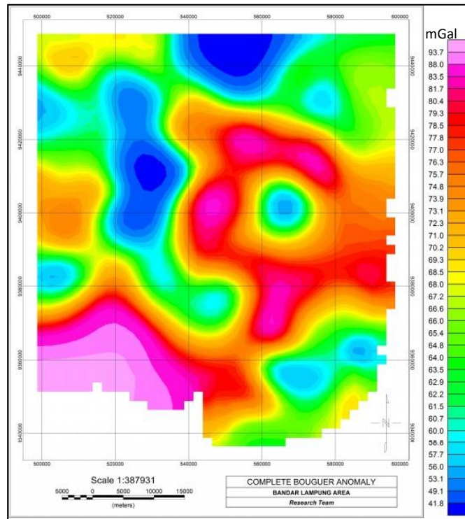
FIGURE 3. Complete Bouguer Anomaly Map of Bandar Lampung City.
