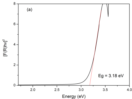
Figure 3. Results of the energy gap sample A.
