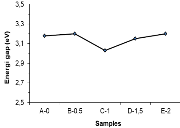
Fig. 4. Energy gap of samples A, B, C, D, and E.
