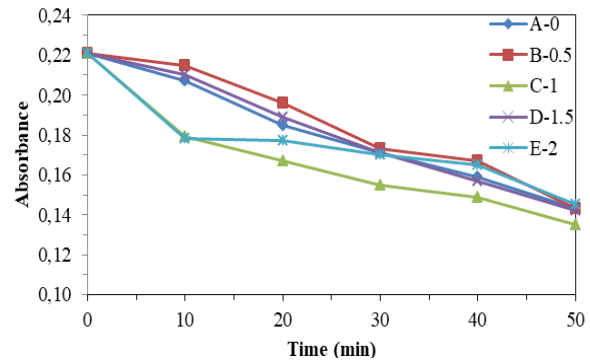
Fig 5. Photodegradation of nanotitania with the addition of ethanolamine under sunlight irradiation on samples A-0, B-0.5, C-1, D-1.5 and E-2 at the peak position \lambda = 411 nm.
