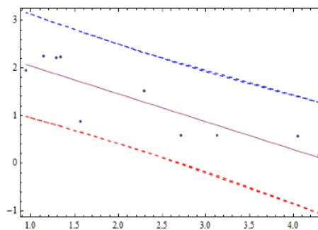
Figure 3. Predicted linear regression curves (middle), regression curves for the upper limit of the confidence interval (top) and the regression curve for the lower limit of the confidence interval (bottom). Source: Mathematica® output
