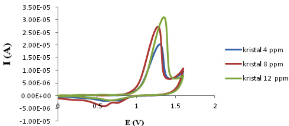
Fig. 7: Cyclic voltammograms of RNV-1 recorded at Pt electrode
