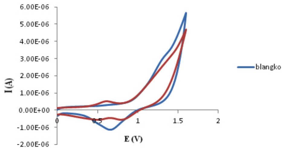
Fig. 5: Cyclic voltammograms of MF recorded at Pt electrode
