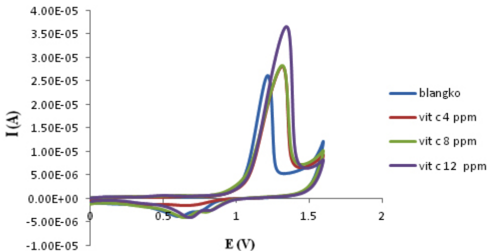
Fig. 8: Cyclic voltammograms of ascorbat acid recorded at Pt electrode
