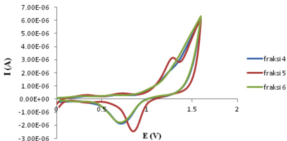
Fig. 6: Cyclic voltammograms of sF-4,5,6 of MF recorded at Pt electrode
