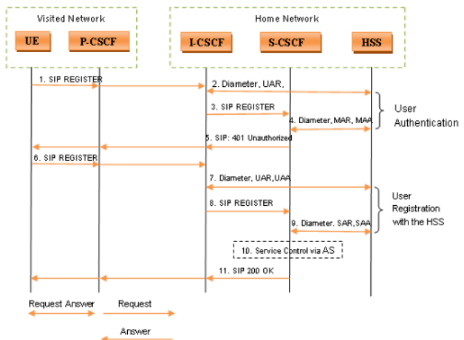
Figure 5. Signalling messages flow in registration procedure
