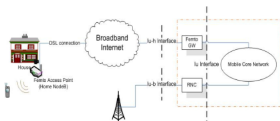
Figure 2. Logical architecture of LTE-based femtocell
