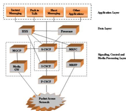
Figure 1. Layer architecture of IMS
