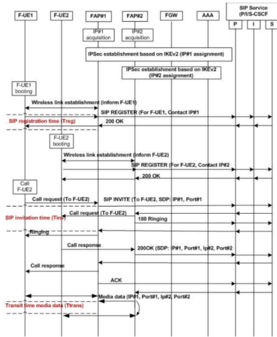
Figure 6. Session establishment signalling in femtocell
