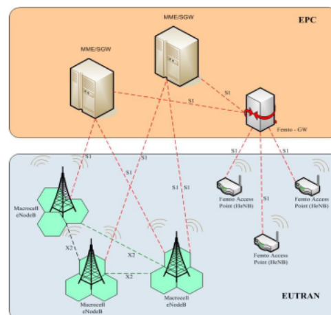
Figure 3. Logical architecture of LTE-A based femtocell
