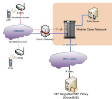
Figure 4. IMS-Femtocell integrated system architecture
