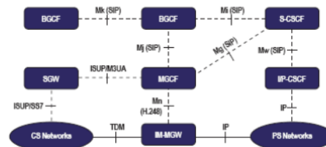
Figure 6. IMS – Circuit Switch interoperability Architecture
