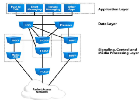
Figure 3. Interact of IMS logical functions
