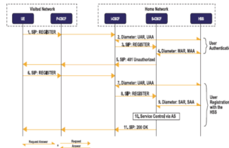
Figure 5. Signalling message flow of registration
