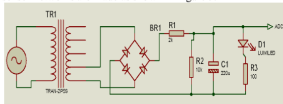
Figure 3. Voltage Sensor Circuit
