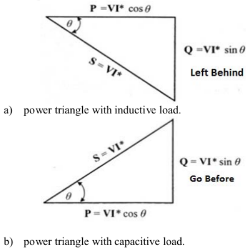
Figure 1. Power Triangle [1]
