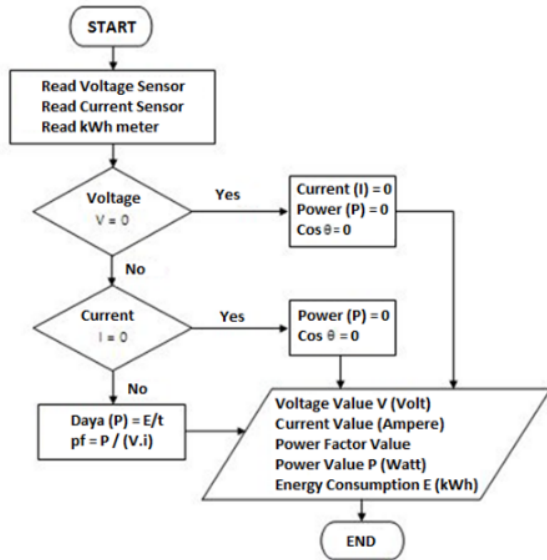
Figure 5. Flow Chart Program.
