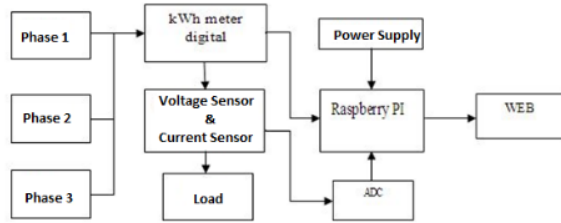
Figure 2. Block Diagram System
