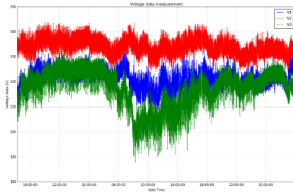
Figure 6. Voltage Monitoring Graphs
