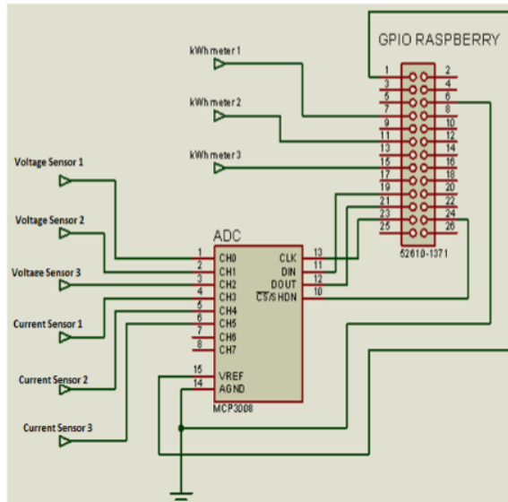
Figure 5. Connection Sensor with Raspberry Pi (BCM2835)
