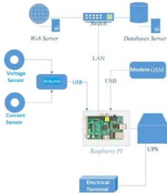
Fig. 1 Hardware Topology Design for Smart Monitoring System
