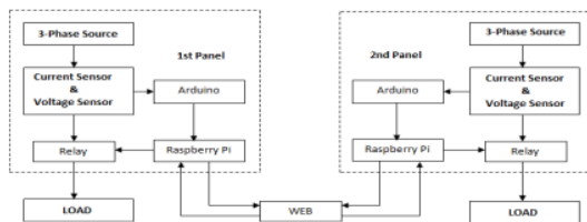
Fig. 2 Block Diagram System
