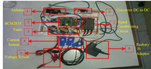
Fig. 3 Hardware Design
