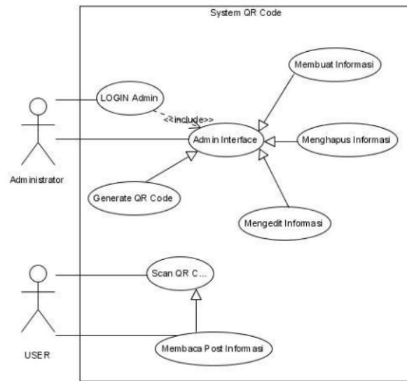
Gambar 2. Use Case Diagram QR Code
