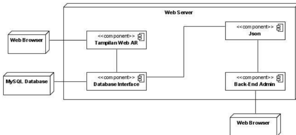
Gambar 3. Deployment Diagram
