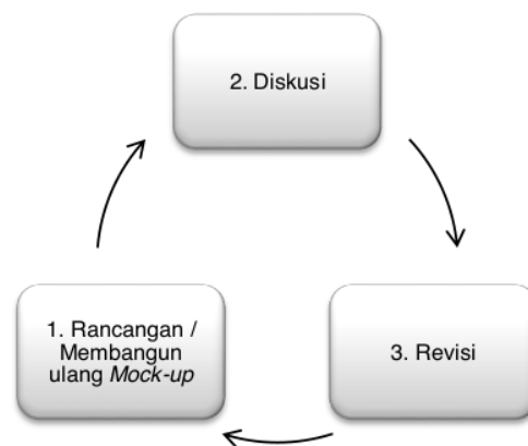
Gambar 1. Metode Prototyping
