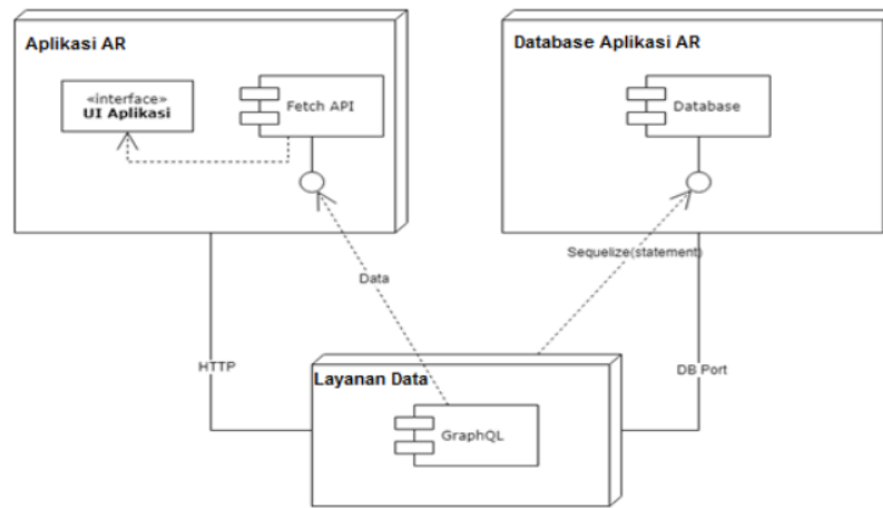
Gambar 14. Deployment Diagram
