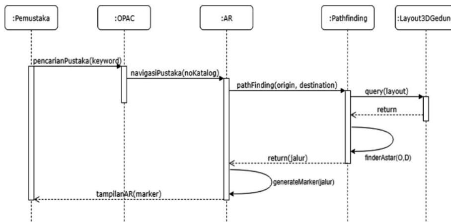
Gambar 4. Sequence Diagram
