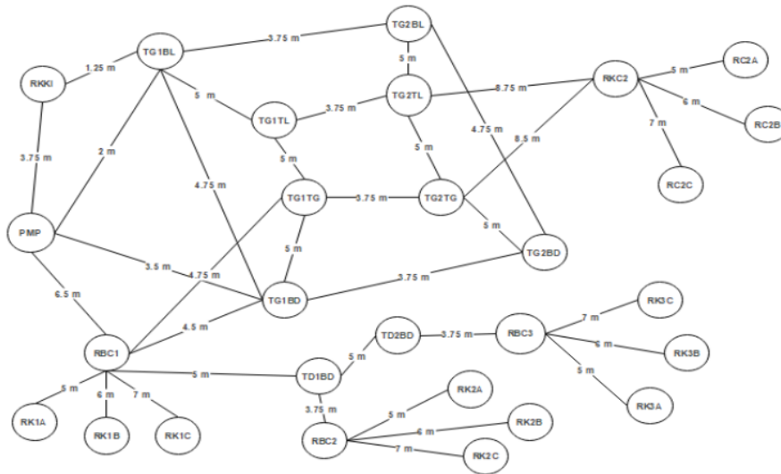
Gambar 6. Graph Diagram
