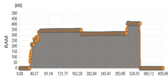
Gambar 12. Grafik Memory Game
