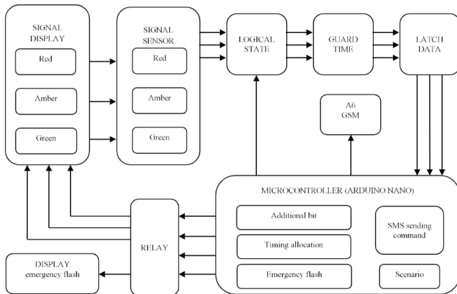
Fig. 2 Devices diagram block
