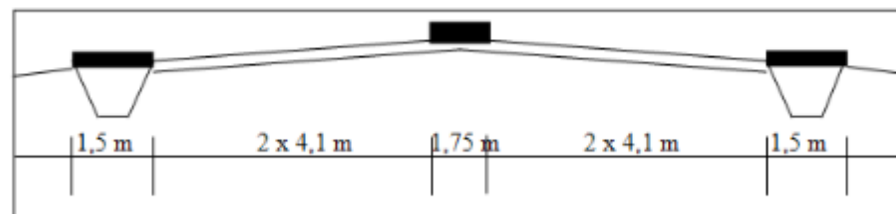
Fig. 3. Cross Section After Road Widening
