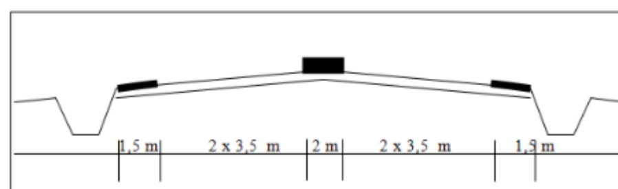
Fig. 2. Cross Section Before Road Widening
