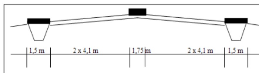
Fig. 6. Sectional Road after Road Widening
