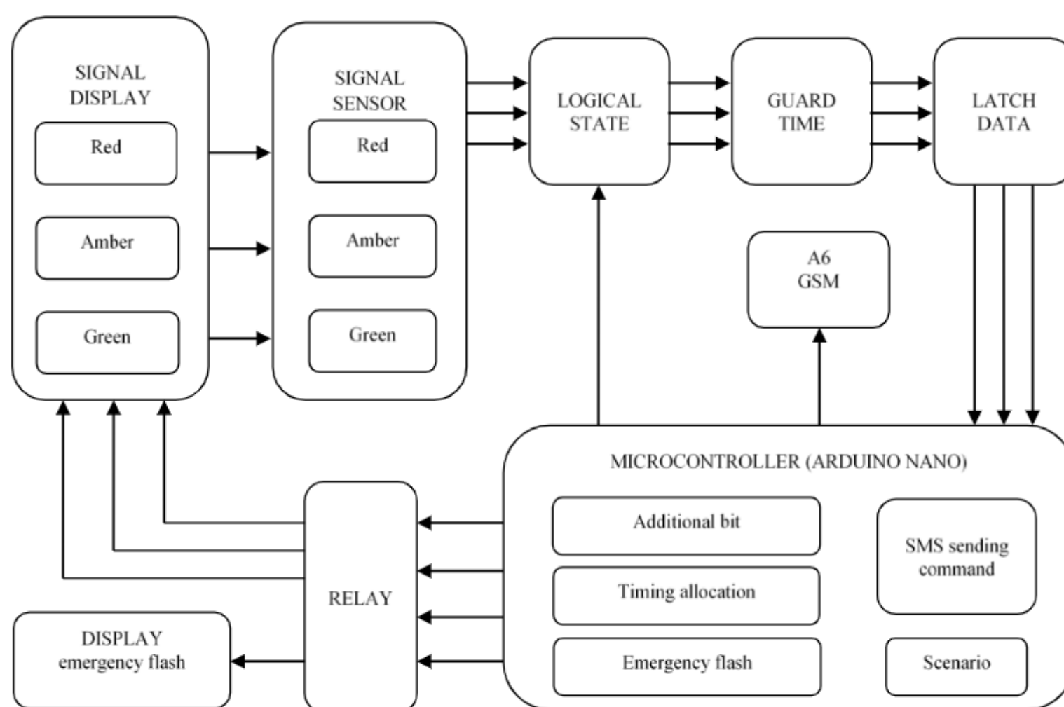
Fig. 2 Devices diagram block
