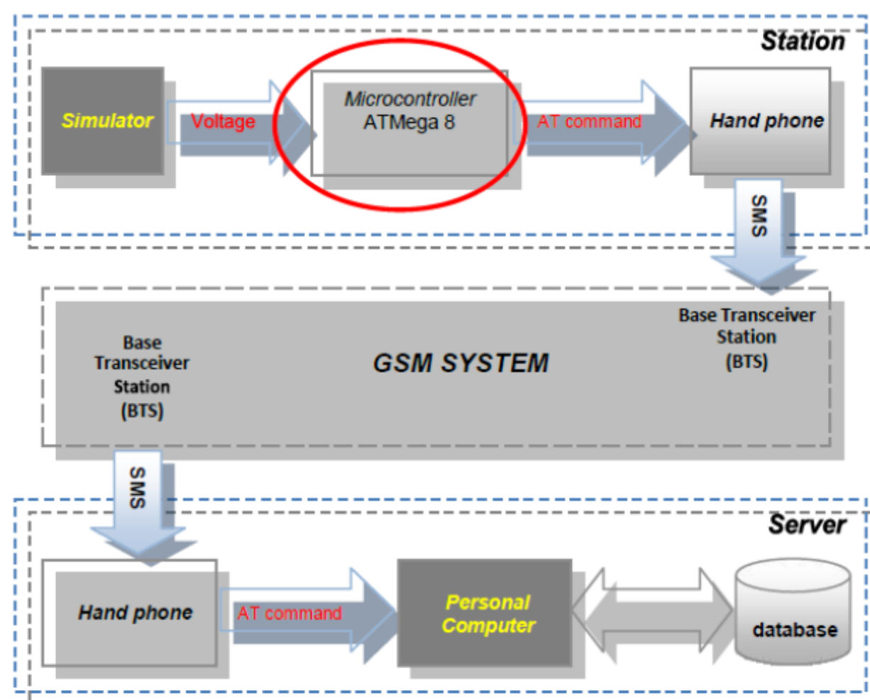
Fig. 5 Self-diagnosis system of traffic light [7]
