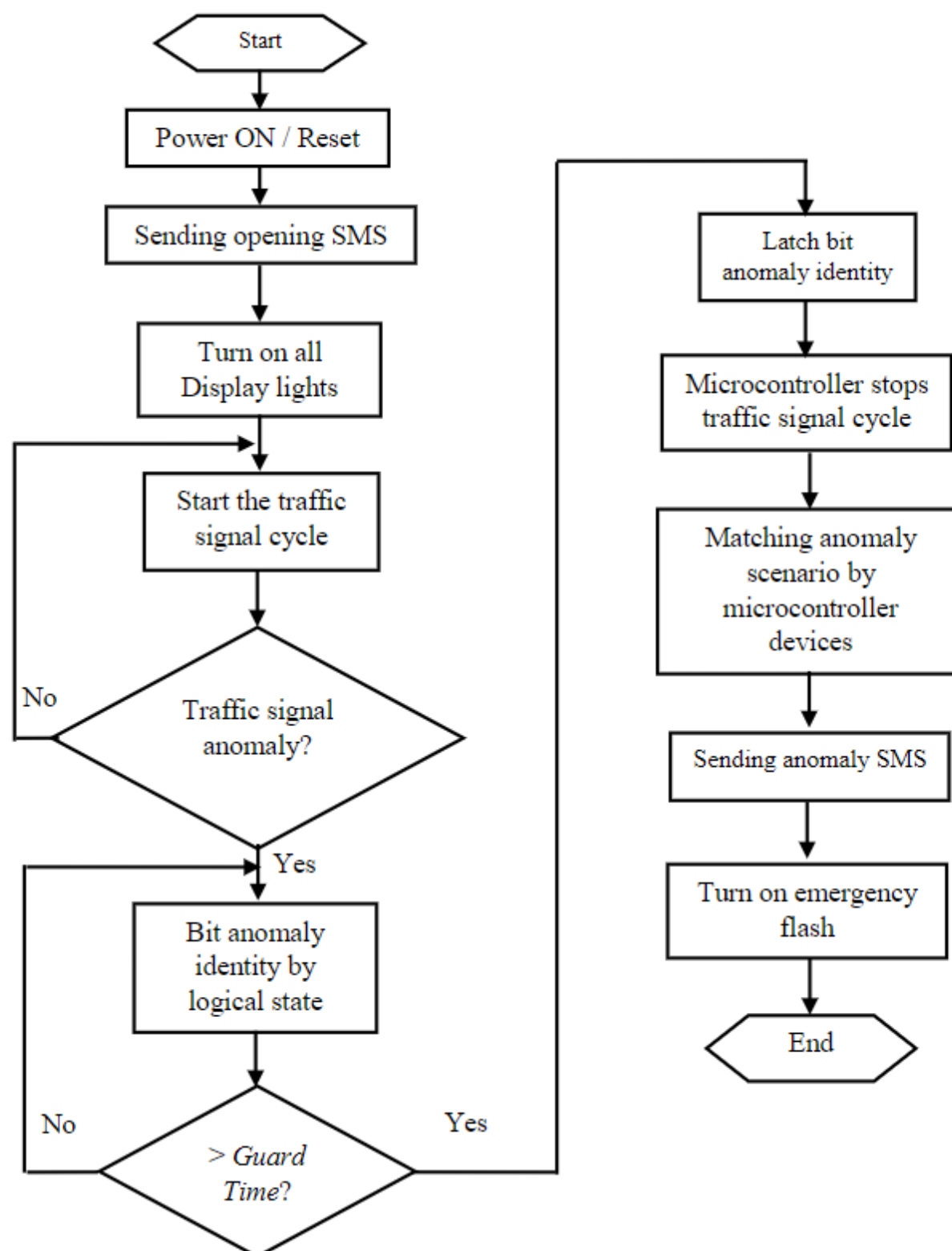
Fig. 4 Flow chart of signal monitoring system
