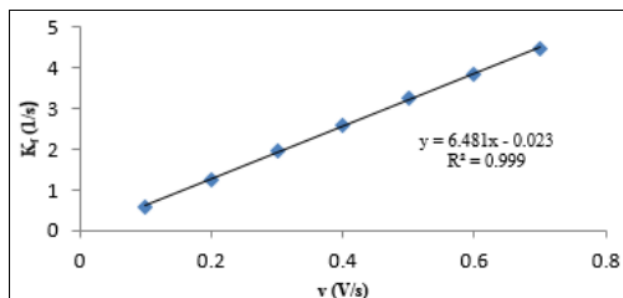
Figure 4. Linear regression curve of k_f against potential scanning rate ( \nu ) of compound 1
