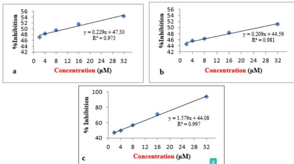
Figure 6. Linear regression curve of antioxidant (a) diphenyltin(IV) di-4-aminobenzoate; (b) triphenyltin(IV) 4-aminobenzoate; (c) ascorbic acid
