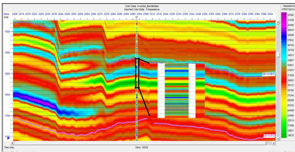
Gambar 13. Hasil inversi LP Sparsespikes
