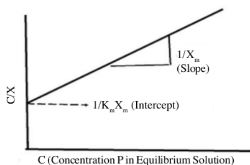
Figure 1. An ideal Langmuir Curve.
