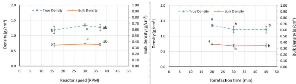
Figure 5. Effect of reactor speed (left) and torrefaction duration (right) on the density of torrefied pellets (points followed by common letters are not statistically different at 5%. Error bars are standard deviation.)
