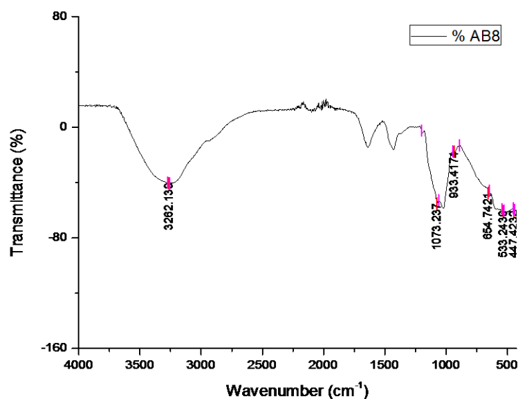
Figure 3. FT-IR spectra of crude extract produced by Streptomyces sp AB8
