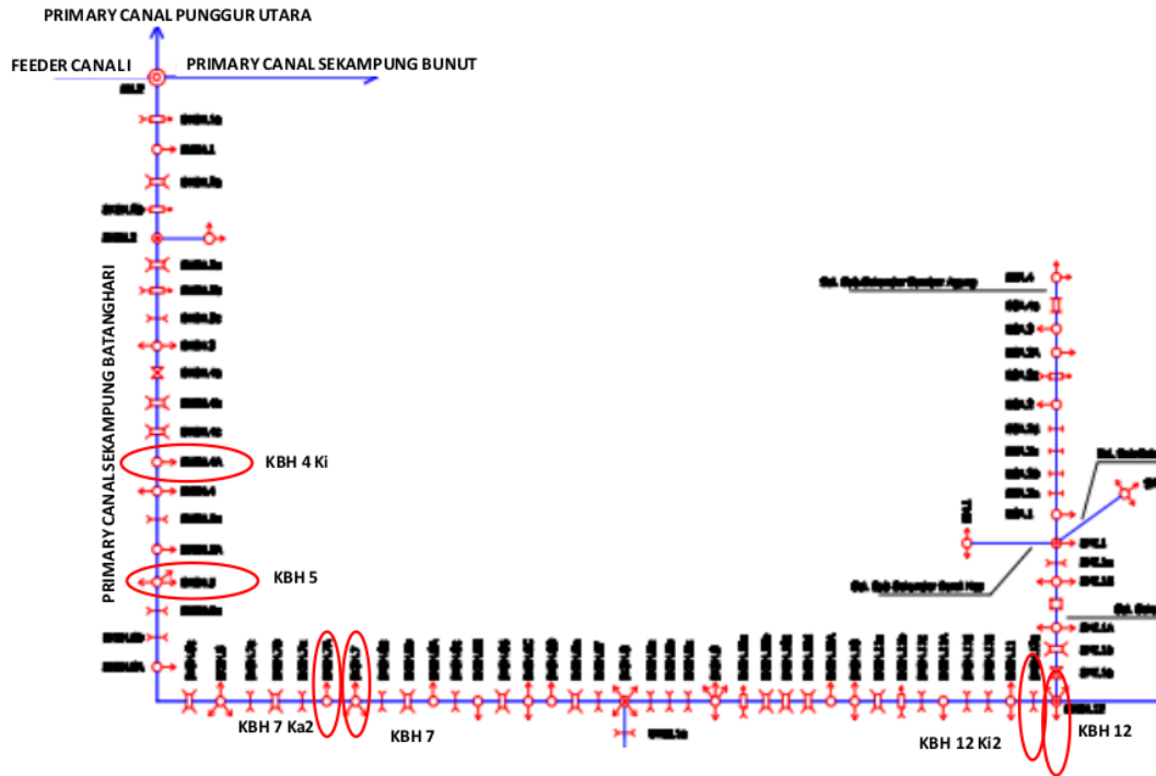
Figure 1. Study area of Sekampung Batanghari irrigation area
