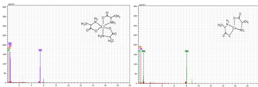
Figure 2. The Results of EDX characterization of complex compounds [Cr(ala)_3] and [Cu(ala)_2]
