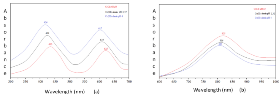
Figure 1. The Results of UV-Vis characterization of complex compounds (a) [Cr(ala)_3] and (b) [Cu(ala)_2]
