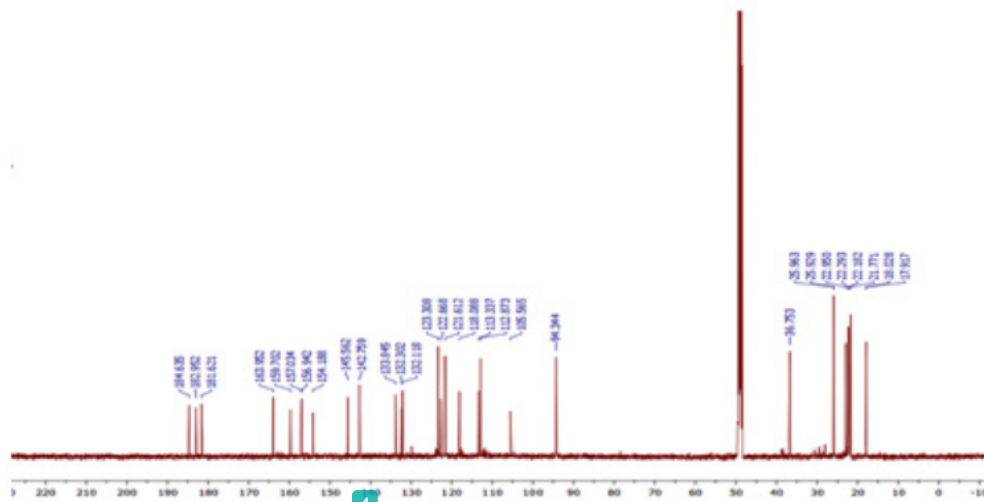
Fig. 2: ^{13}\text{C} NMR spectrum of isolated compound 1
