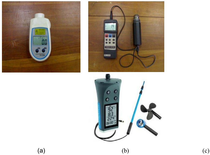
Figure 3. Photograph of measurement instruments: a. tacho meter, b. torque meter, and c. propeller flow meter
