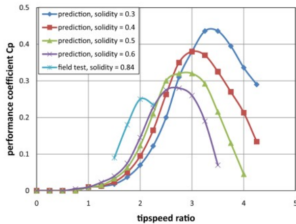
Figure 7. Predicted and measured performance of Darrieus HKTs of varying solidity
