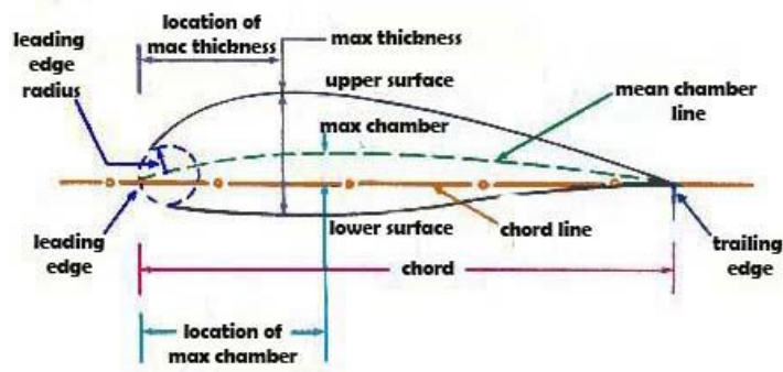
Figure 6. Parameters of NACA airfoil
