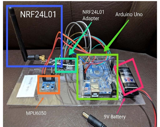
Fig. 5. The prototype of sensor and sink nodes.
