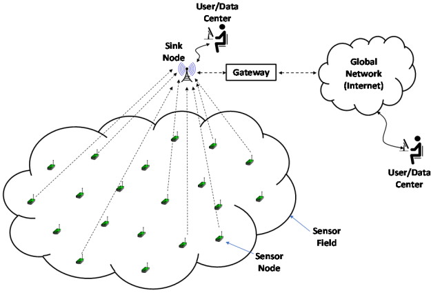
Fig. 1. The architecture of wireless sensor network.
