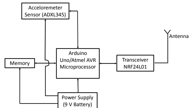
Fig. 3. The architecture of sensor node.
