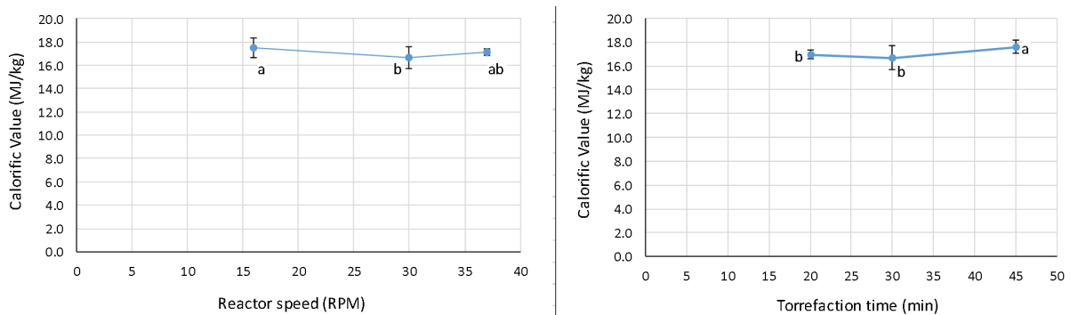
Figure 9. Effect of RPM (left) and torrefaction duration (right) on the calorific value of torrefied pellets. (Points followed by common letters are not statistically different at 5%. Error bars are standard deviation.)
