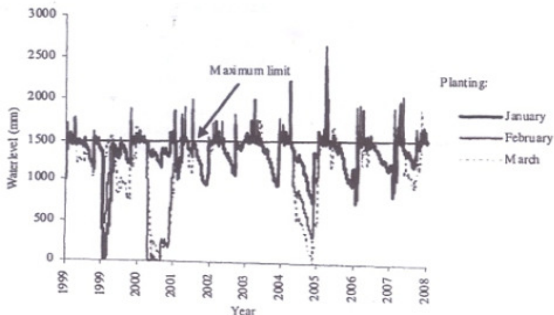
Figure 4. Pond water level.
