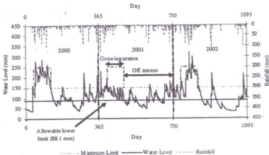
Figure 3. Field water levels and rainfall for February planting in 2000, 2001, and 2002.
